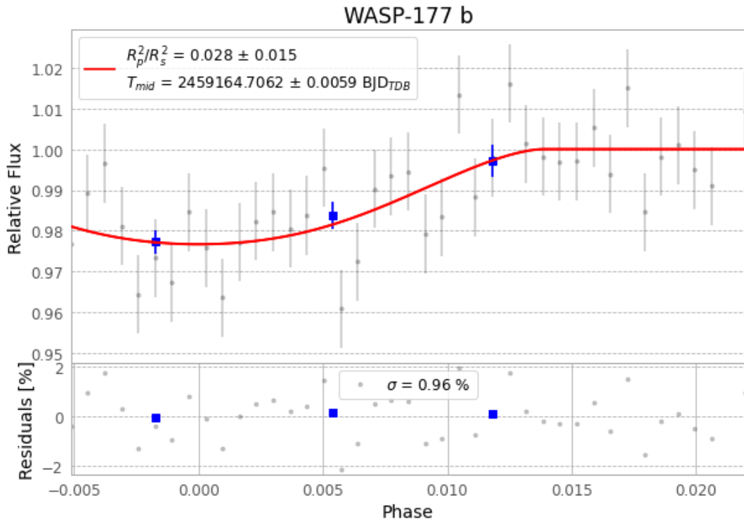
Figure 1 — FinalLightCurve_WASP-177 b_2020-11-10.png (SHA-256 0219a11e14744ef0...)
