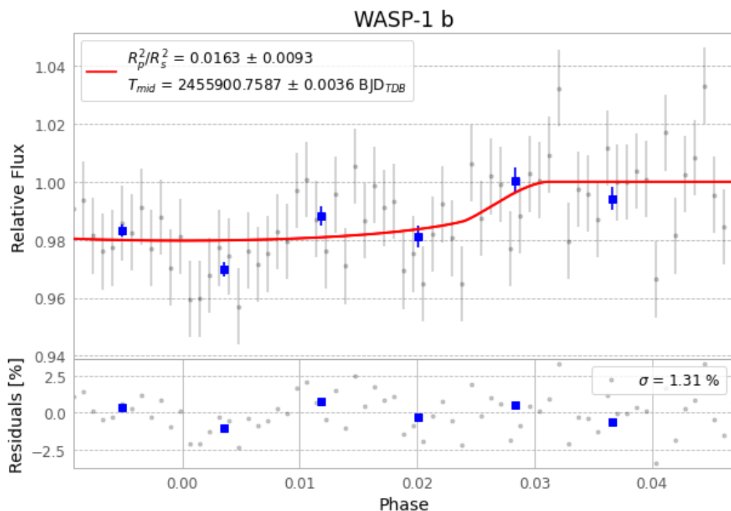
Figure 1 — FinalLightCurve_WASP-1 b_2011-12-04.png (SHA-256 3cfa25cd00ce1ba3...)
