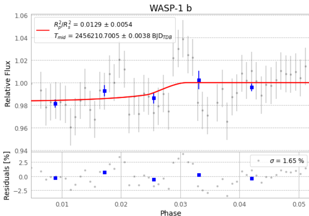
Figure 1 — FinalLightCurve_WASP-1 b_2012-10-09.png (SHA-256 a93227c838bd8504...)
