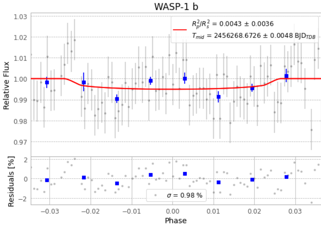
Figure 1 — FinalLightCurve_WASP-1 b_2012-12-06.png (SHA-256 10eed87a16154516...)
