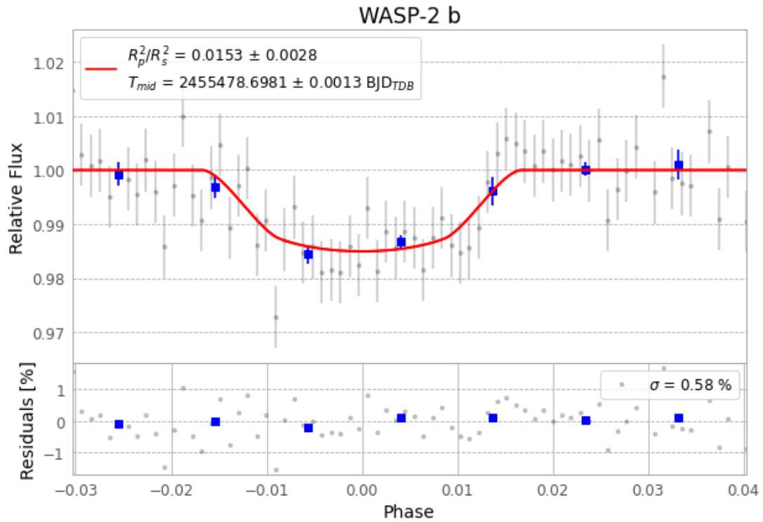
Figure 1 — FinalLightCurve_WASP-2 b_2010-10-08.png (SHA-256 260a86237dce4010...)
