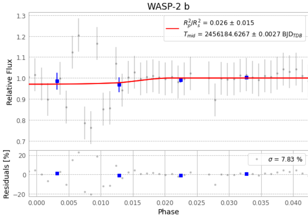
Figure 1 — FinalLightCurve_WASP-2 b_2012-09-13.png (SHA-256 4bd73689abb9d361...)
