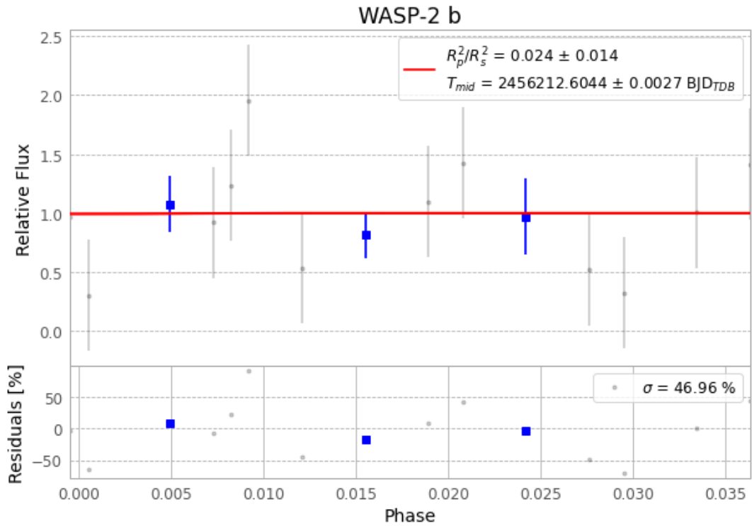
Figure 1 — FinalLightCurve_WASP-2 b_2012-10-11.png (SHA-256 48382996c102f0b2...)
