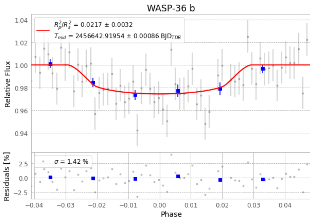
Figure 1 — FinalLightCurve_WASP-36 b_2013-12-16.png (SHA-256 e3db2f85078e025a...)
