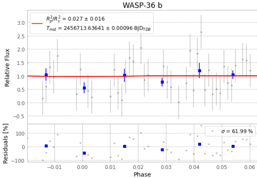
Figure 1 — FinalLightCurve_WASP-36 b_2014-02-24.png (SHA-256 b4a9c2fc4aaa3455...)
