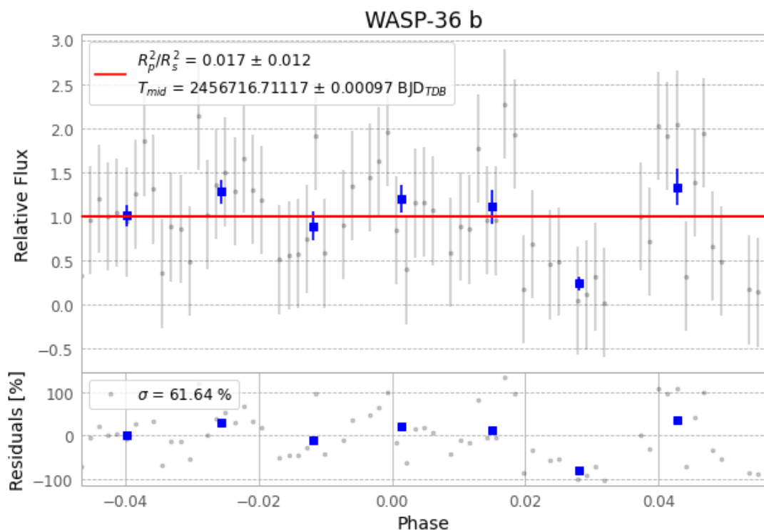
Figure 1 — FinalLightCurve_WASP-36 b_2014-02-27.png (SHA-256 2680fdb35e9676f...)
