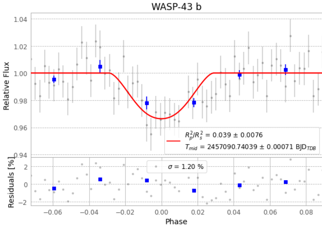
Figure 1 — FinalLightCurve_WASP-43 b_2015-03-08.png (SHA-256 352250891358a3f2...)
