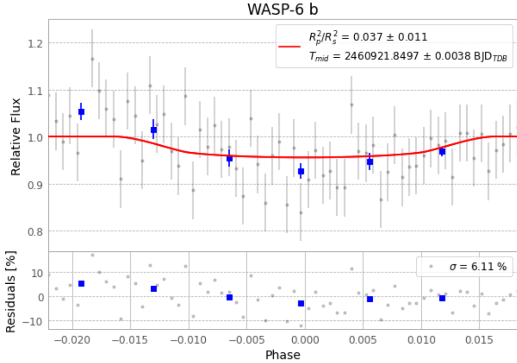
Figure 1 — FinalLightCurve_WASP-6 b_2025-09-02.png (SHA-256 9cacf0eaf9bc6a3a...)
