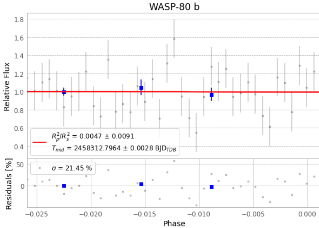
Figure 1 — FinalLightCurve_WASP-80 b_2018-07-12.png (SHA-256 cc17617f1ecb12f0...)
