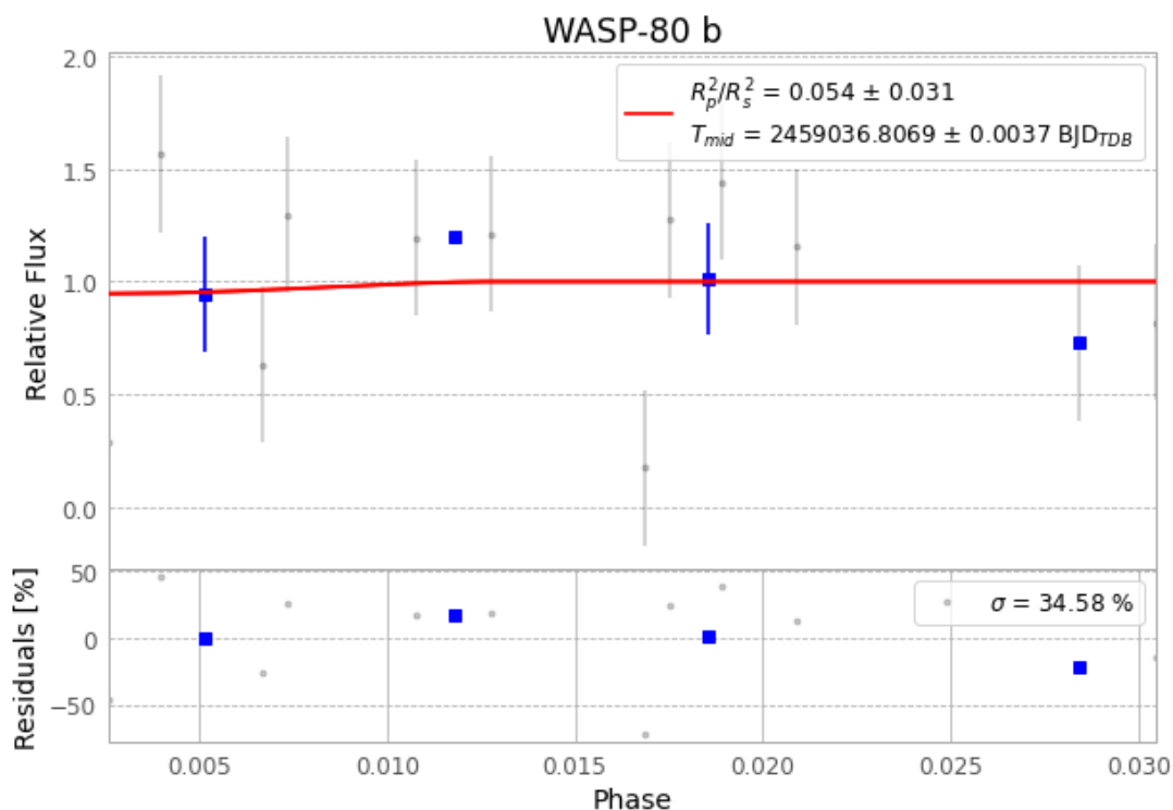
Figure 1 — FinalLightCurve_WASP-80 b_2020-07-06.png (SHA-256 8d720aeb805869bf...)
