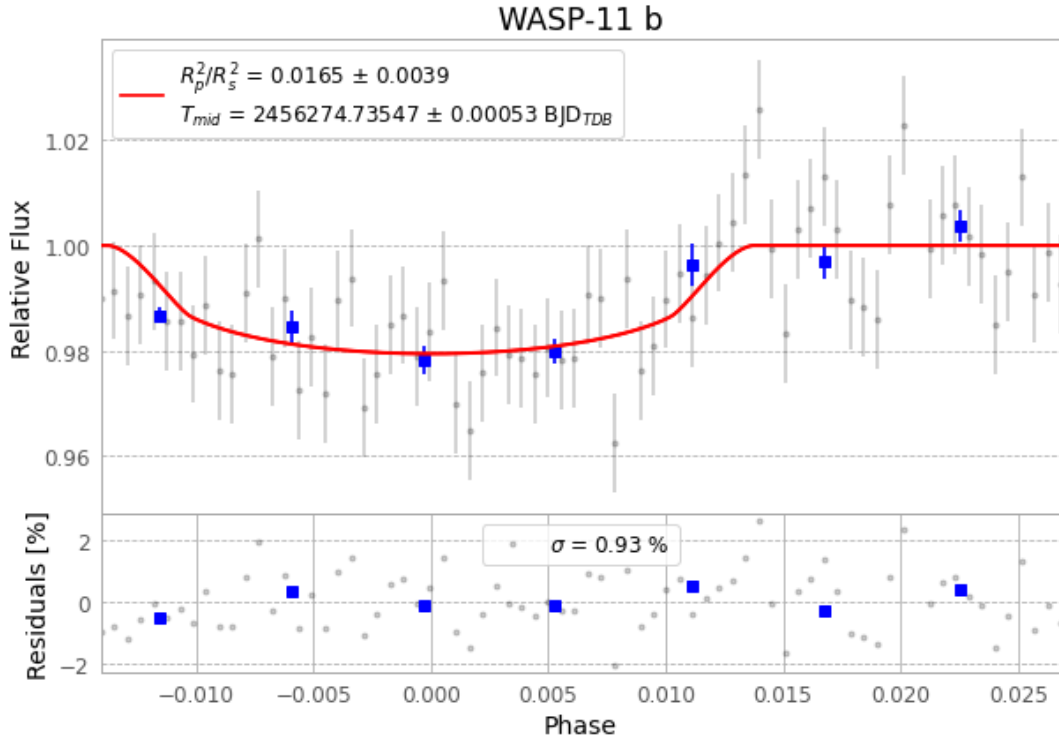
Figure 1 — FinalLightCurve_WASP-11 b_2012-12-12.png (SHA-256 f6ee4eef08e7a7f5...)
