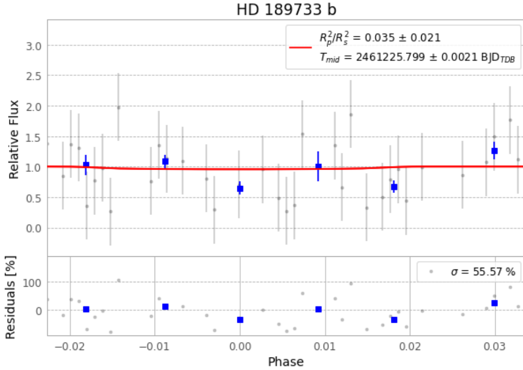
Figure 1 — FinalLightCurve_HD 189733 b_2026-07-03.png (SHA-256 b29ee4b1f35f6e99...)
