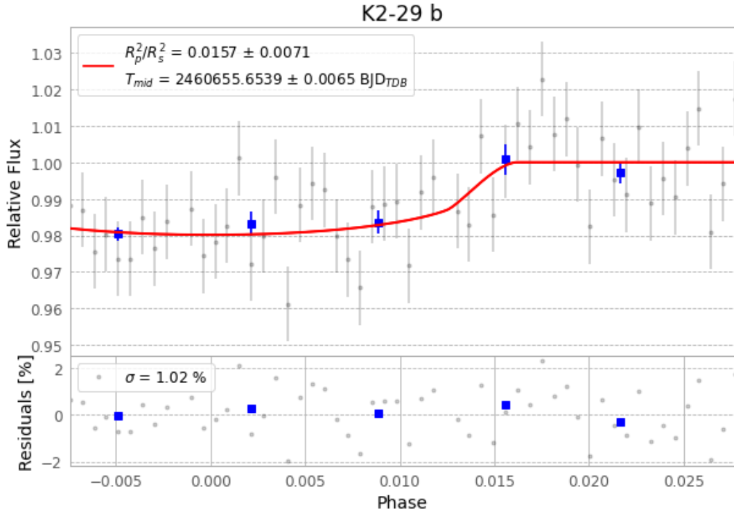
Figure 1 — FinalLightCurve_K2-29 b_2024-12-10.png (SHA-256 142d9092d07fbce0...)
