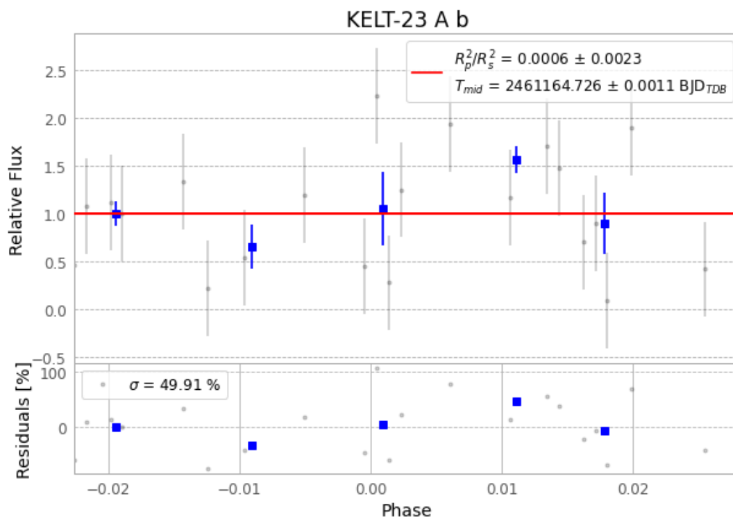
Figure 1 — FinalLightCurve_KELT-23 A b_2026-05-03.png (SHA-256 91682b77ccc47a9a...)
