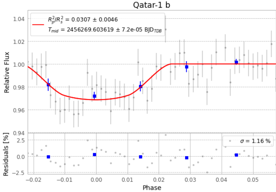
Figure 1 — FinalLightCurve_Qatar-1 b_2012-12-07.png (SHA-256 0dfb65c9389179d5...)
