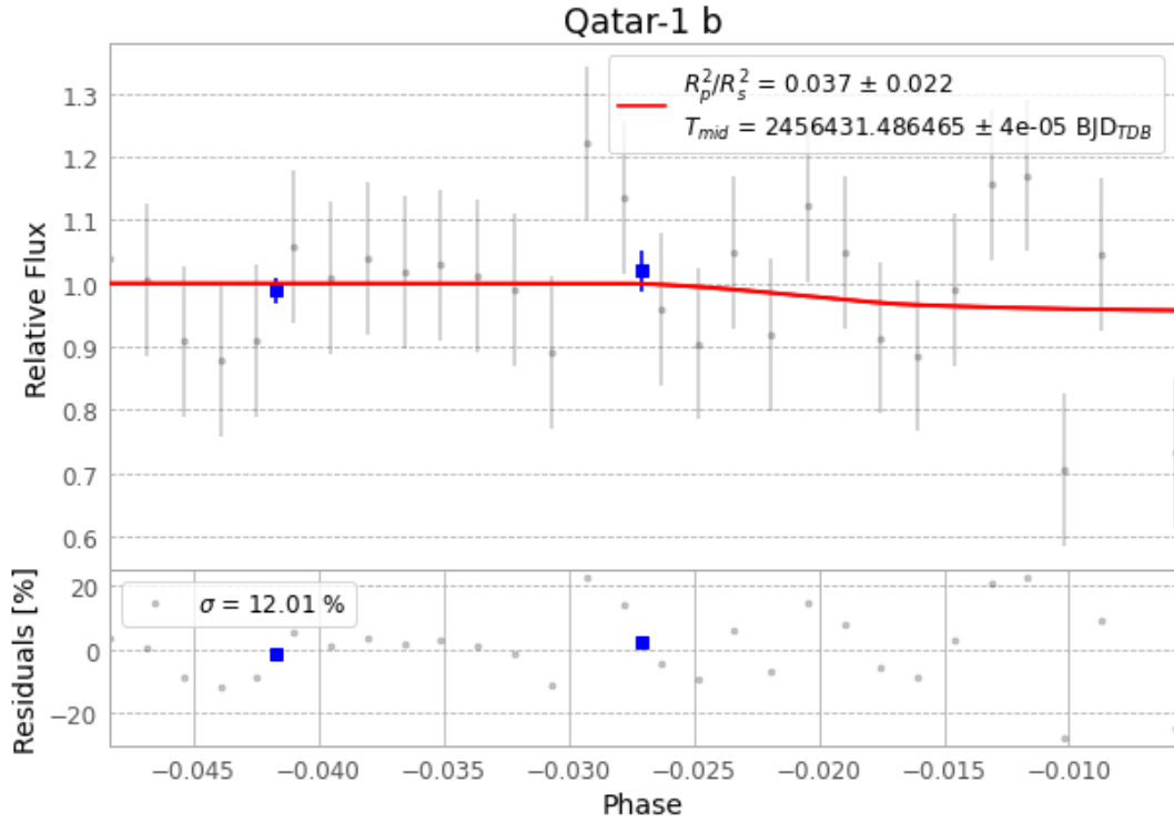
Figure 1 — FinalLightCurve_Qatar-1 b_2013-05-20.png (SHA-256 966f58219495012b...)
