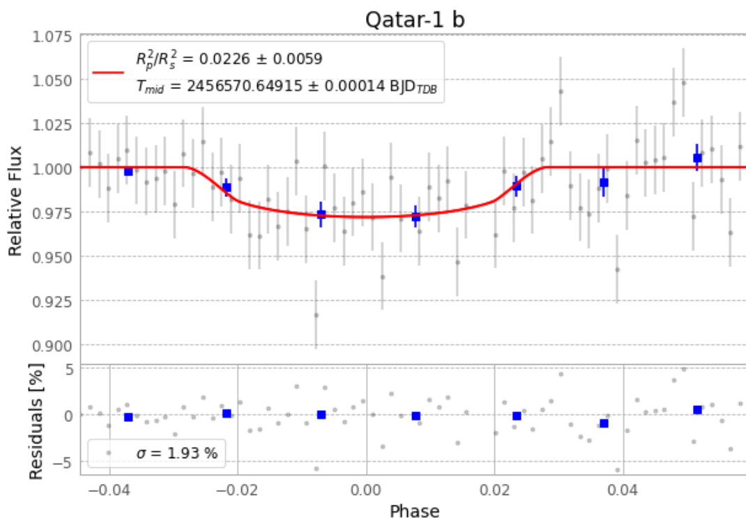
Figure 1 — FinalLightCurve_Qatar-1 b_2013-10-04.png (SHA-256 1f5b6e0e730e287f...)
