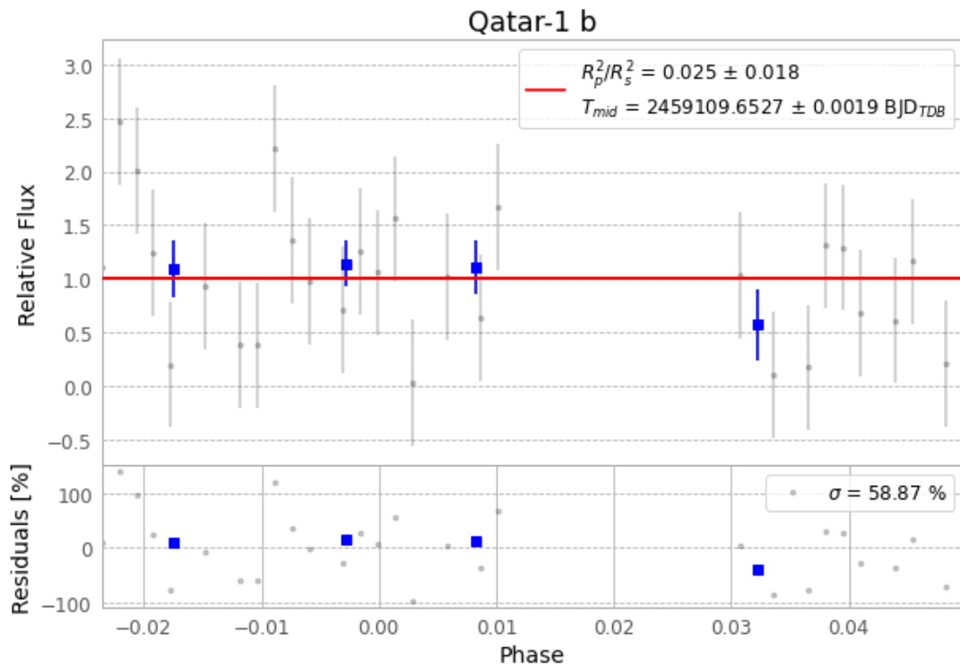
Figure 1 — FinalLightCurve_Qatar-1 b_2020-09-16.png (SHA-256 8d5b8487d80c04a0...)
