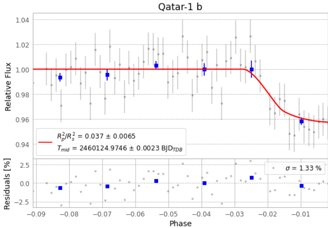
Figure 1 — FinalLightCurve_Qatar-1 b_2023-06-29.png (SHA-256 6dee8cff47417511...)
