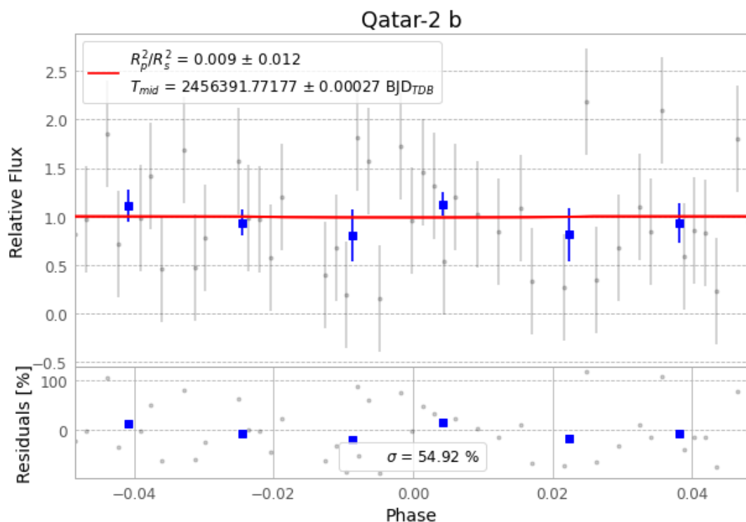
Figure 1 — FinalLightCurve_Qatar-2 b_2013-04-08.png (SHA-256 6000a1fb39ccdc2c...)
