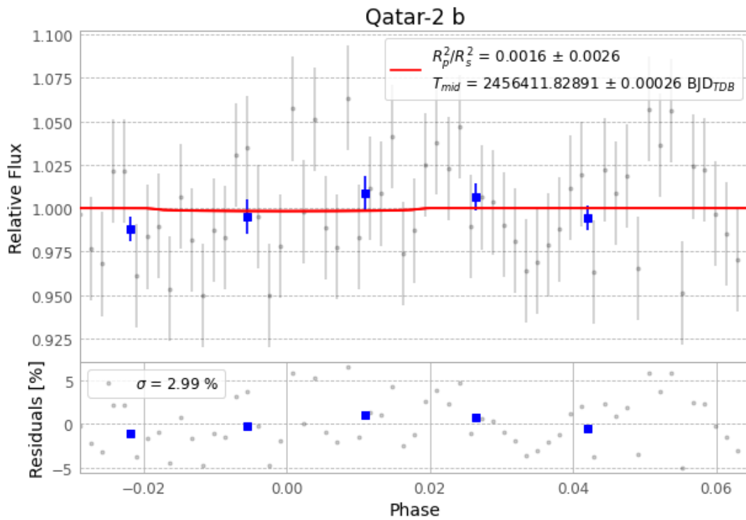
Figure 1 — FinalLightCurve_Qatar-2 b_2013-04-28.png (SHA-256 ed21e4579973d203...)
