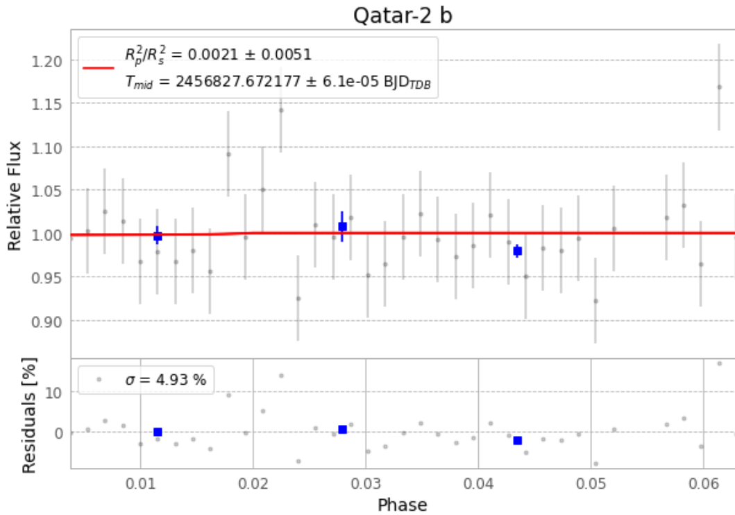
Figure 1 — FinalLightCurve_Qatar-2 b_2014-06-18.png (SHA-256 96c2a7d8a4208d83...)
