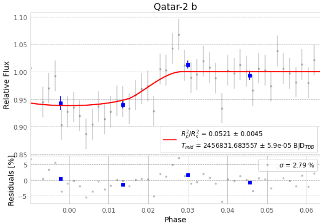
Figure 1 — FinalLightCurve_Qatar-2 b_2014-06-22.png (SHA-256 a43c86d4a123f24b...)
