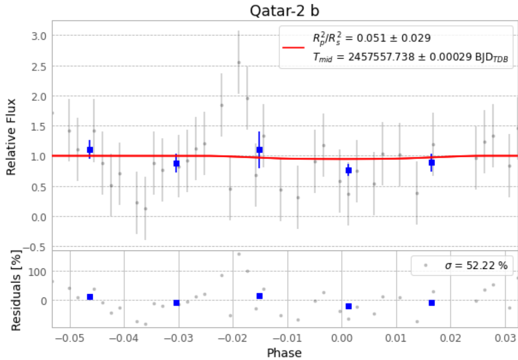
Figure 1 — FinalLightCurve_Qatar-2 b_2016-06-17.png (SHA-256 f18ba04fd4950a46...)
