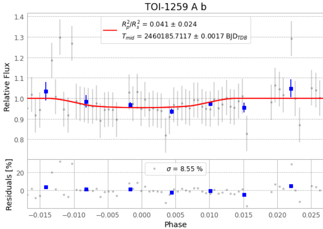
Figure 1 — FinalLightCurve_TOI-1259 A b_2023-08-28.png (SHA-256 daf8cfcb6b3e034d...)
