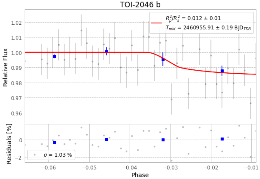
Figure 1 — FinalLightCurve_TOI-2046 b_2025-10-07.png (SHA-256 a07e6d9c1aebce8a...)
