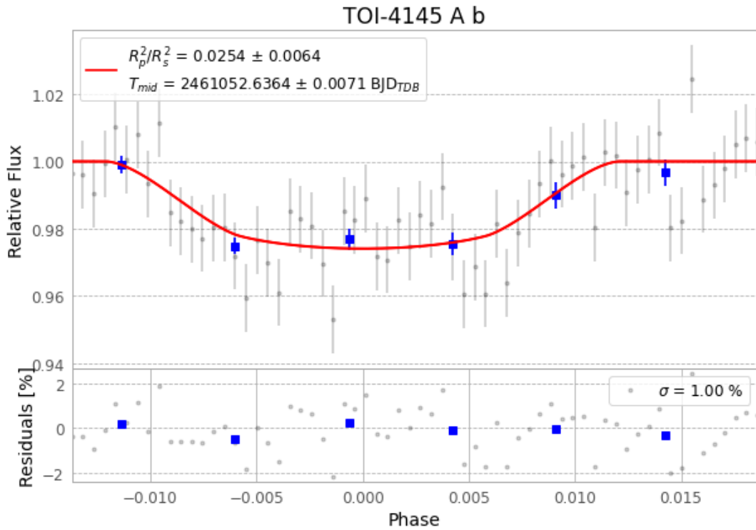
Figure 1 — FinalLightCurve_TOI-4145 A b_2026-01-11.png (SHA-256 d964b18f2a778a7e...)
