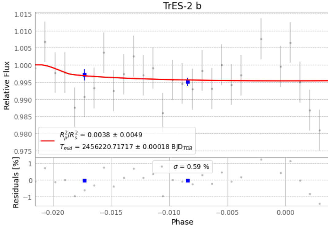
Figure 1 — FinalLightCurve_TrES-2 b_2012-10-19.png (SHA-256 675388fafdb801ae...)
