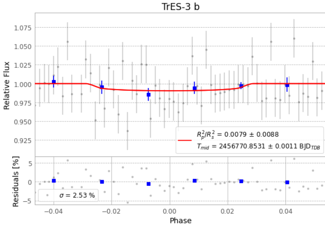
Figure 1 — FinalLightCurve_TrES-3 b_2014-04-22.png (SHA-256 228b0b63c3fa51b6...)
