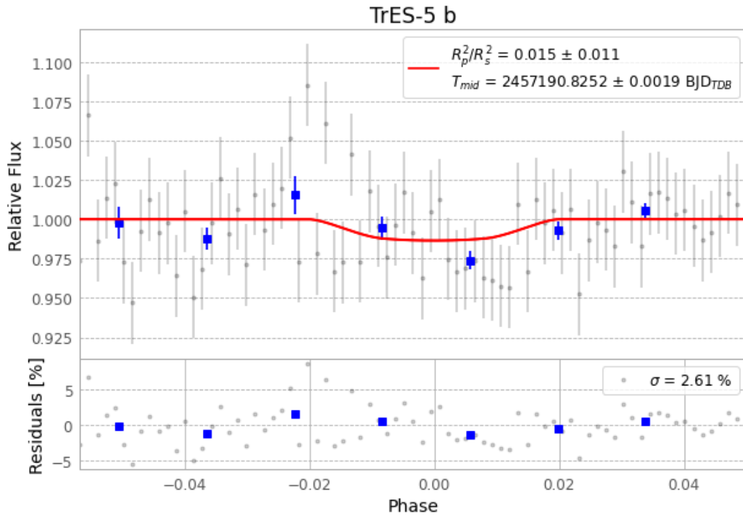
Figure 1 — FinalLightCurve_TrES-5 b_2015-06-16.png (SHA-256 3263a92ce80dc431...)
