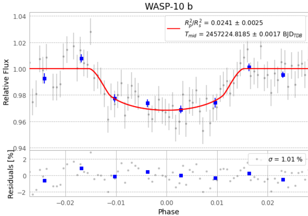
Figure 1 — FinalLightCurve_WASP-10 b_2015-07-20.png (SHA-256 6c6b924fa871711d...)
