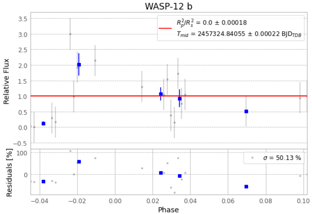
Figure 1 — FinalLightCurve_WASP-12 b_2015-10-28.png (SHA-256 5e67c76952ffcf8d...)
