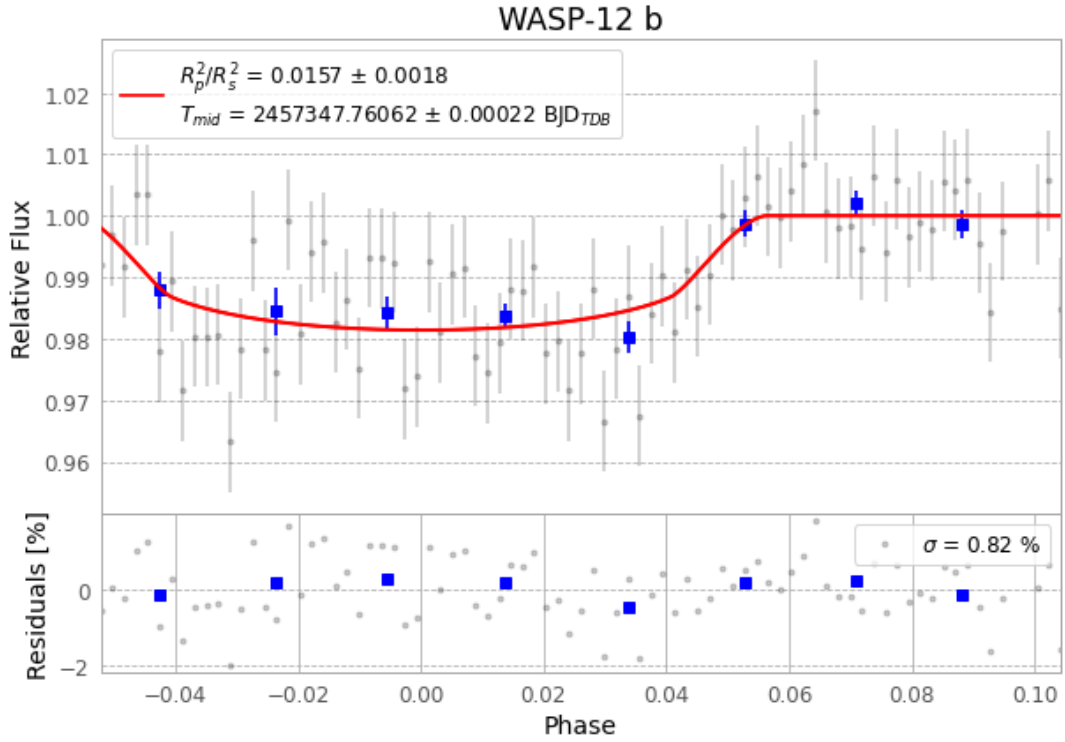
Figure 1 — FinalLightCurve_WASP-12 b_2015-11-20.png (SHA-256 e75c2f8f17de3e74...)
