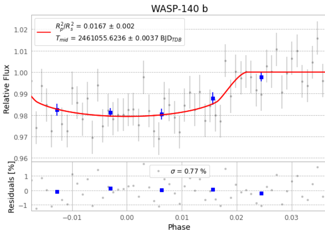
Figure 1 — FinalLightCurve_WASP-140 b_2026-01-14.png (SHA-256 14c6b0b01bc8abba...)
