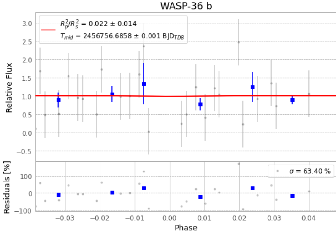
Figure 1 — FinalLightCurve_WASP-36 b_2014-04-08.png (SHA-256 75c440db5017454f...)
