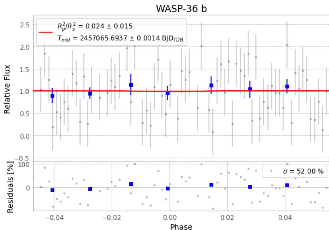
Figure 1 — FinalLightCurve_WASP-36 b_2015-02-11.png (SHA-256 6fe9f8d68aa60168...)
