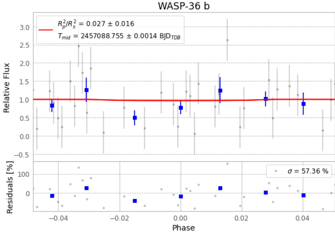
Figure 1 — FinalLightCurve_WASP-36 b_2015-03-06.png (SHA-256 a03bc8e27bb04149...)
