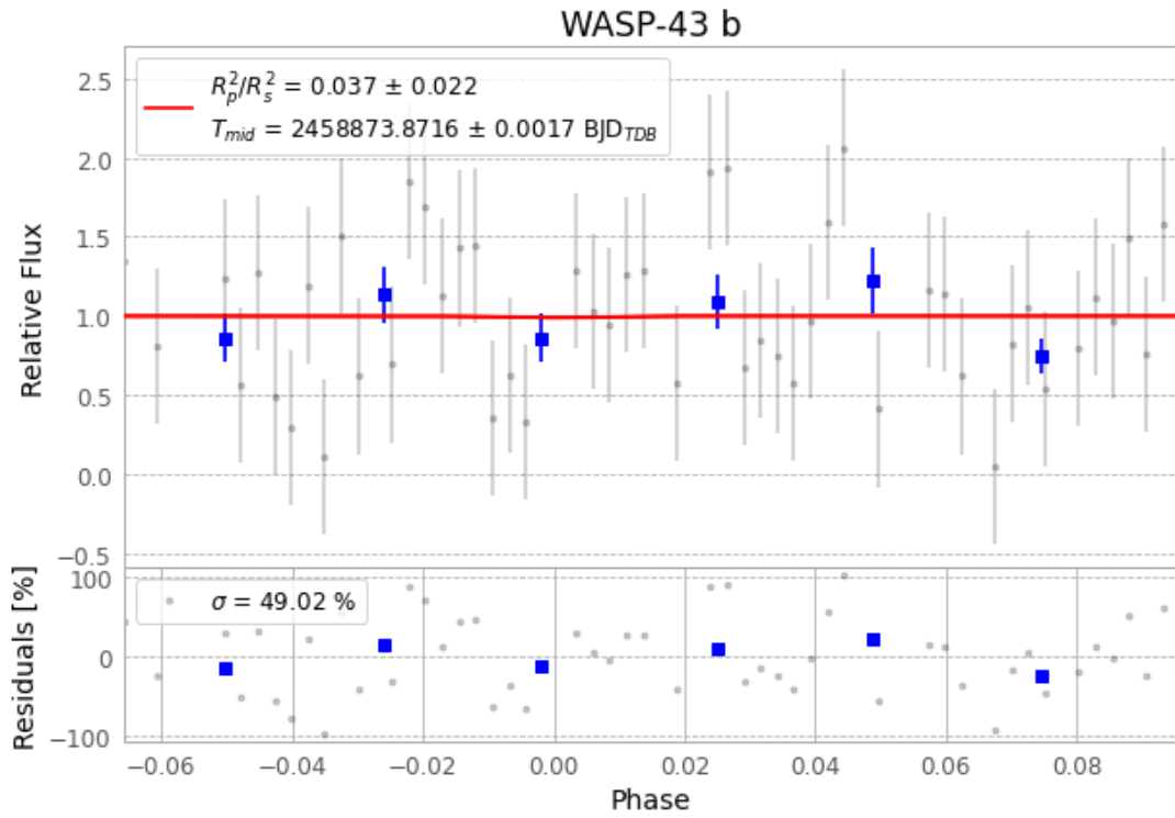
Figure 1 — FinalLightCurve_WASP-43 b_2020-01-25.png (SHA-256 b946391f4d88f461...)
