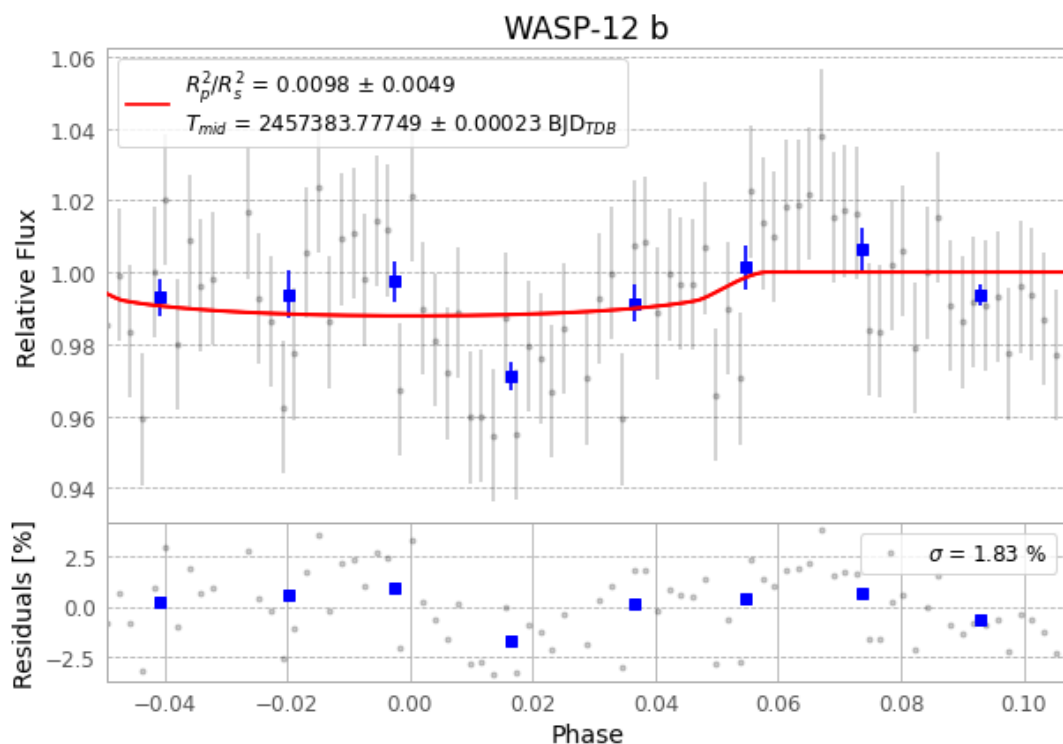
Figure 1 — FinalLightCurve_WASP-12 b_2015-12-26.png (SHA-256 2f40978bc6788b1e...)
