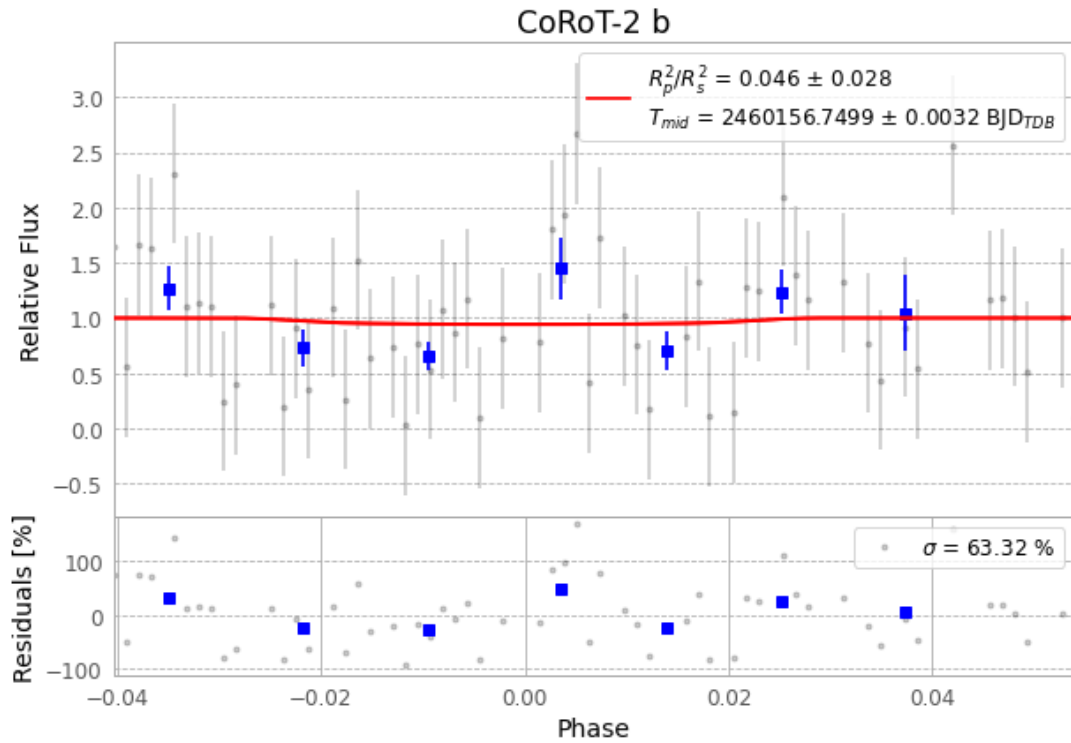
Figure 1 — FinalLightCurve_CoRoT-2 b_2023-07-30.png (SHA-256 2b9a43fb0cc7cb0a...)
