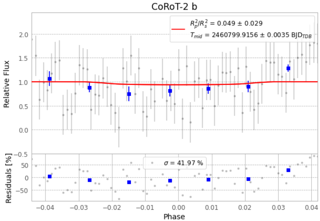
Figure 1 — FinalLightCurve_CoRoT-2 b_2025-05-04.png (SHA-256 bdd313def6ba0be2...)
