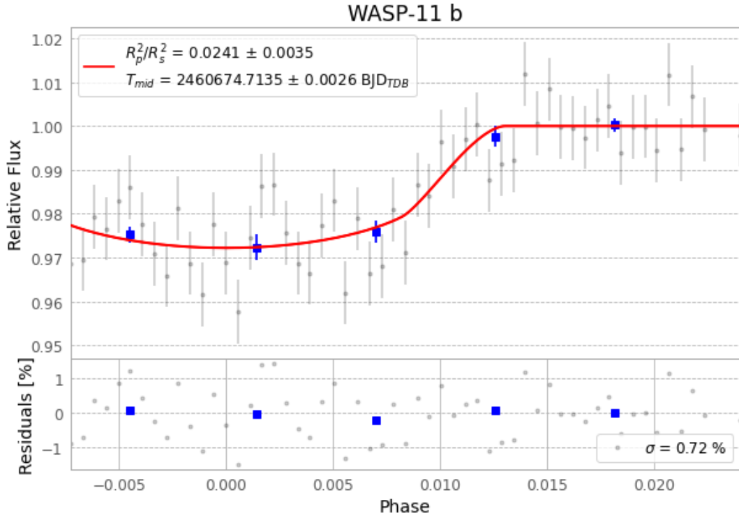
Figure 1 — FinalLightCurve_WASP-11 b_2024-12-29.png (SHA-256 7fdac10d86e855d7...)
