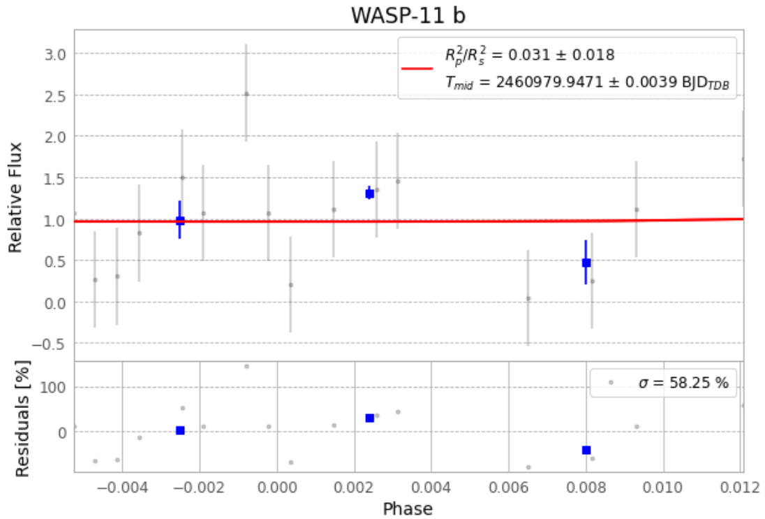
Figure 1 — FinalLightCurve_WASP-11 b_2025-10-31.png (SHA-256 914608dae13be343...)
