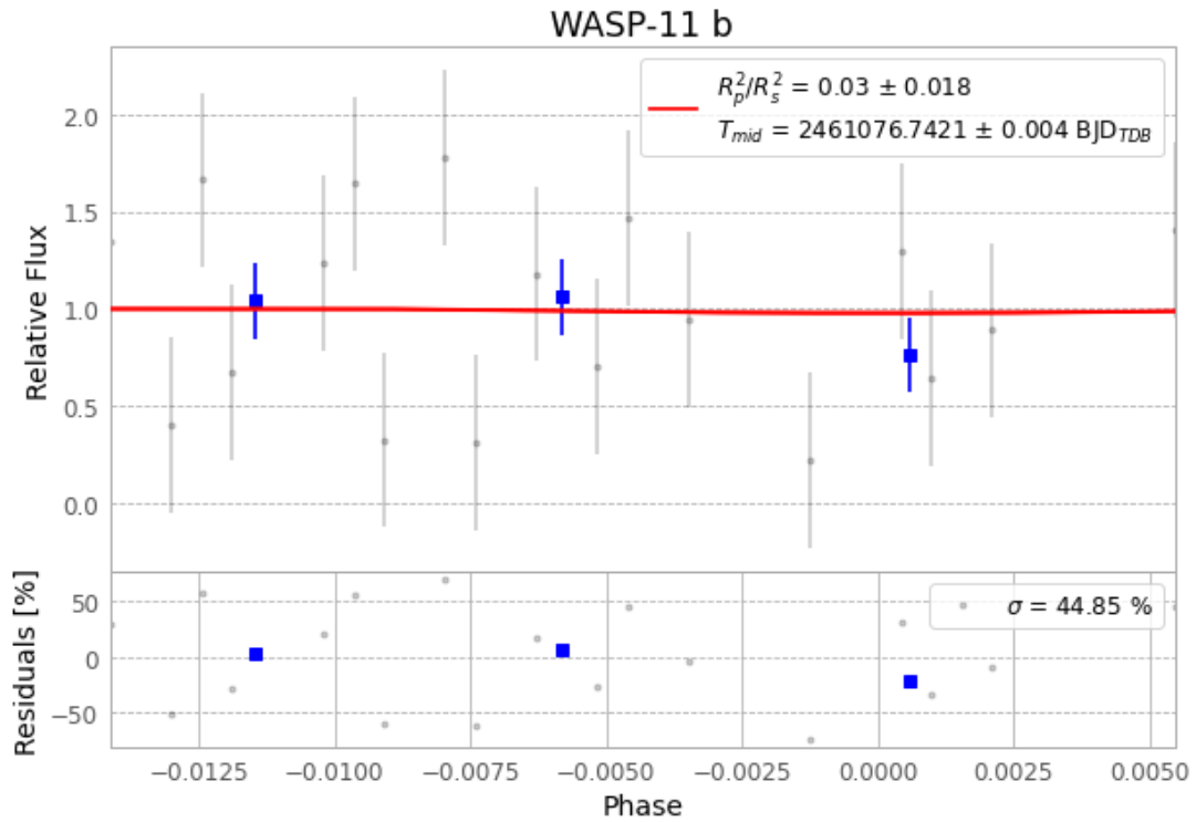
Figure 1 — FinalLightCurve_WASP-11 b_2026-02-04.png (SHA-256 fb10c86ed8ff781c...)
