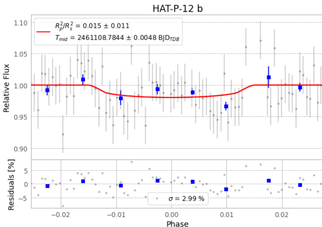
Figure 1 — FinalLightCurve_HAT-P-12 b_2026-03-08.png (SHA-256 dcc80ad94787f600...)
