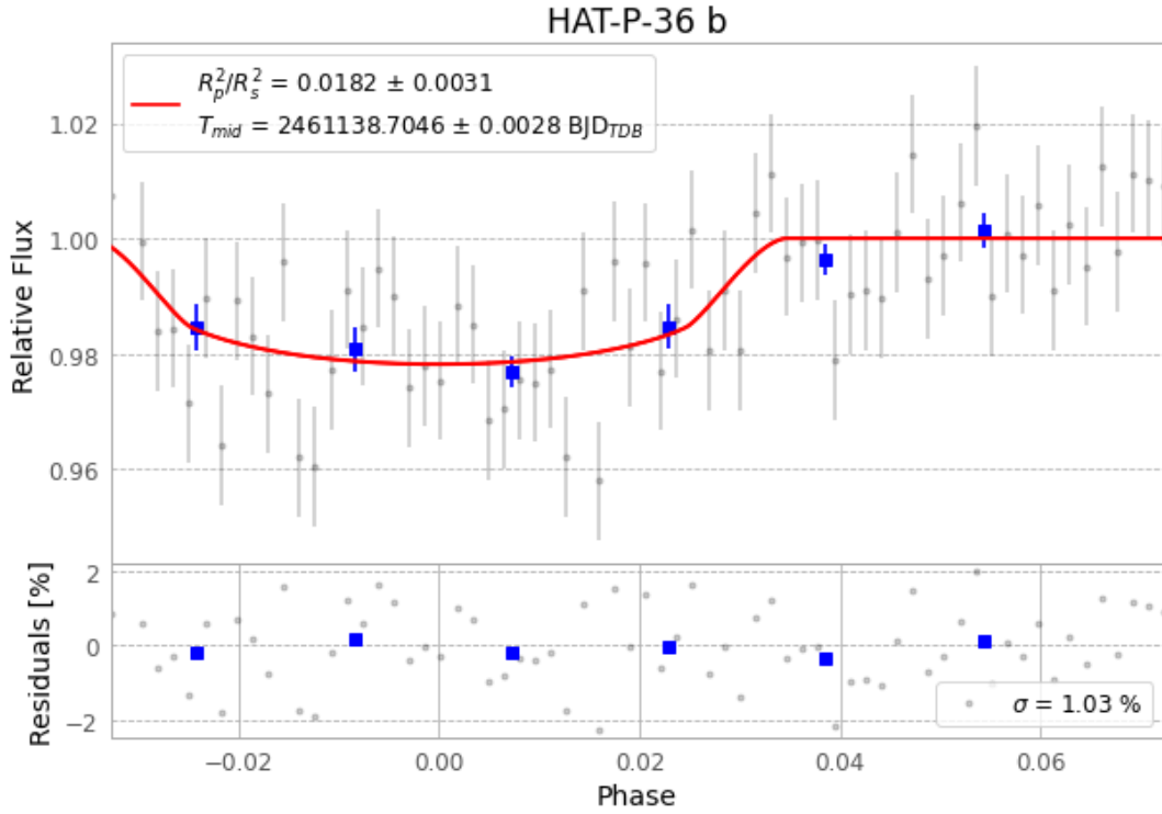
Figure 1 — FinalLightCurve_HAT-P-36 b_2026-04-07.png (SHA-256 beef3b11c2c8a050...)
